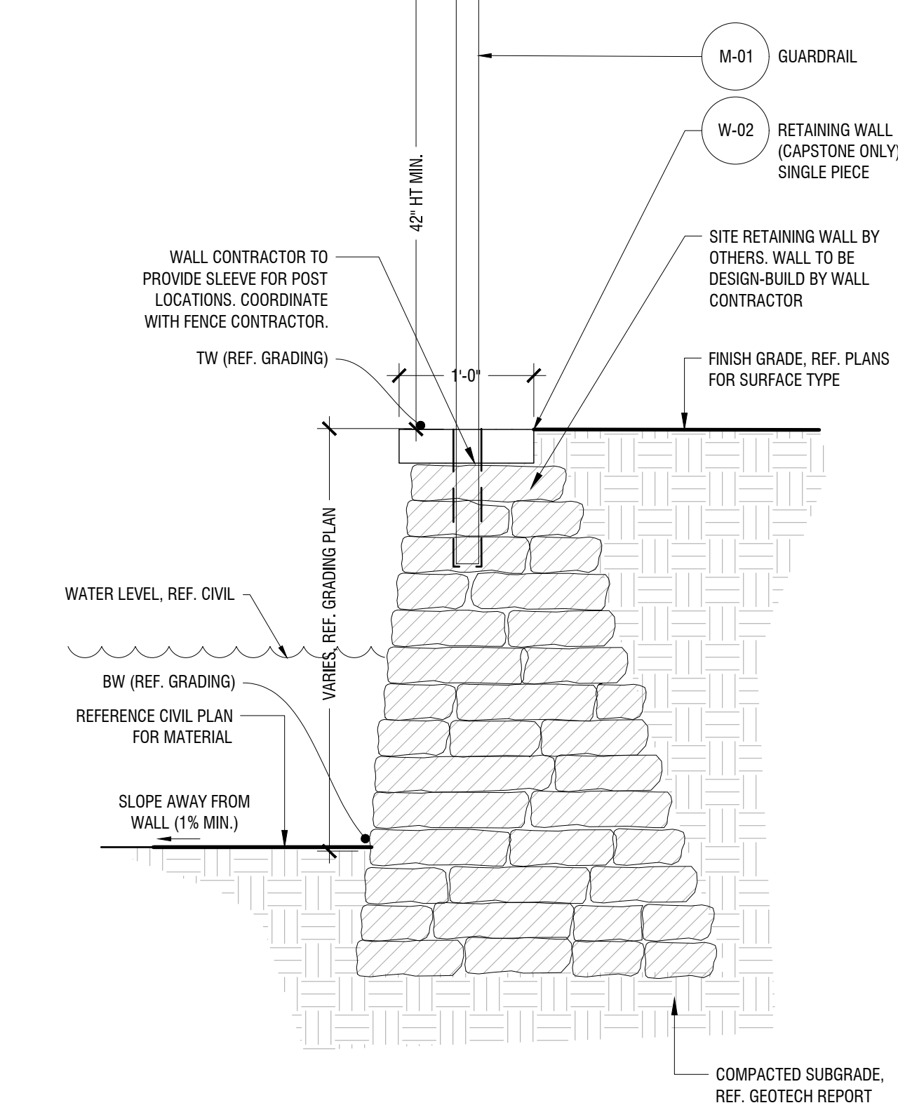
ENGINEERED RETAINING WALL
