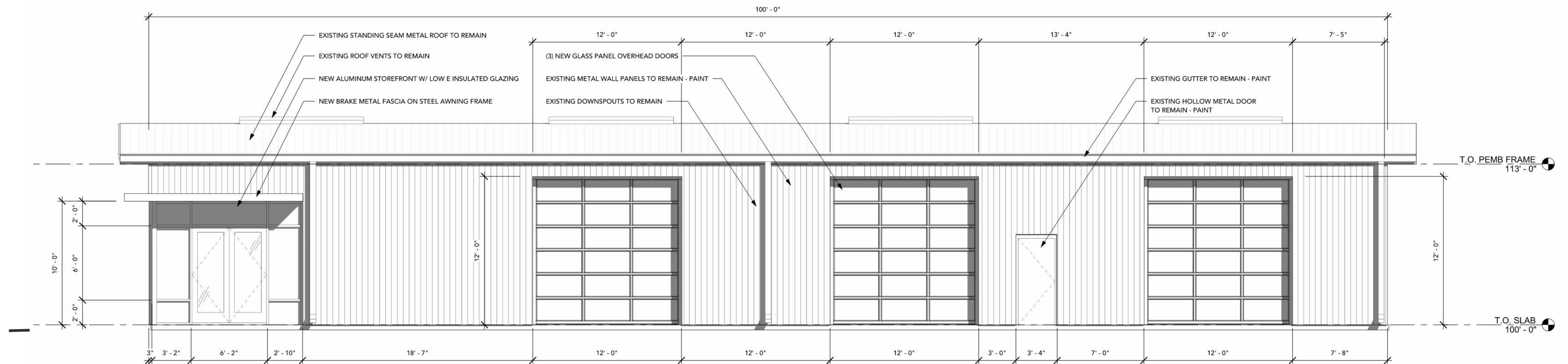
PROPOSED NORTH ELEVATION
