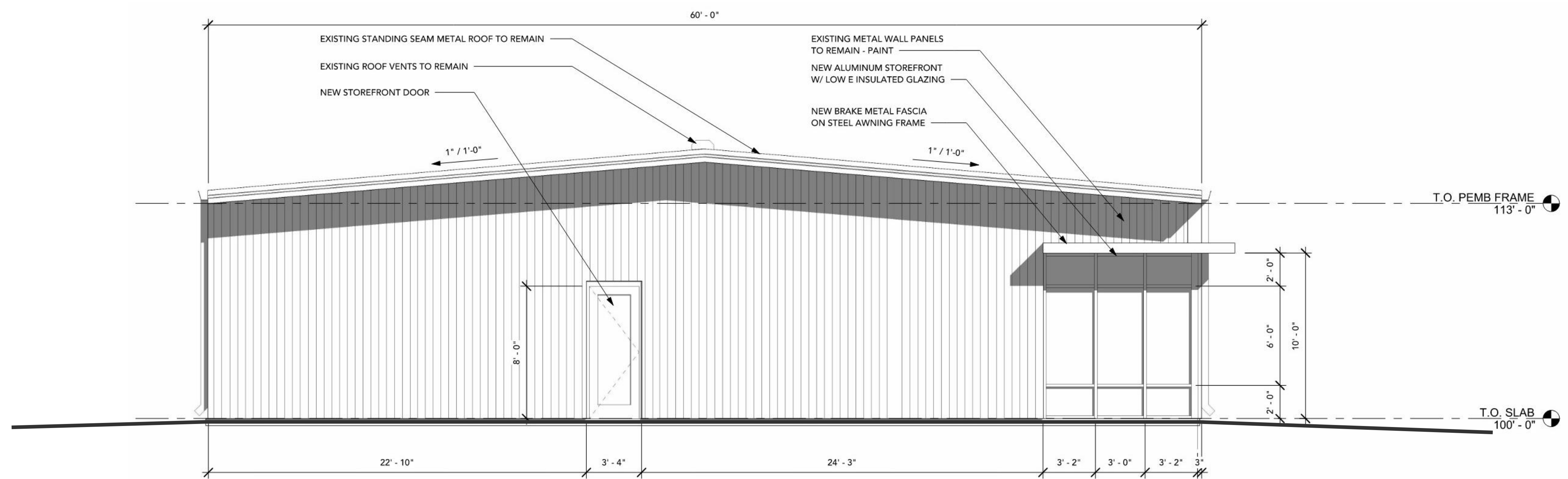
PROPOSED EAST ELEVATION
