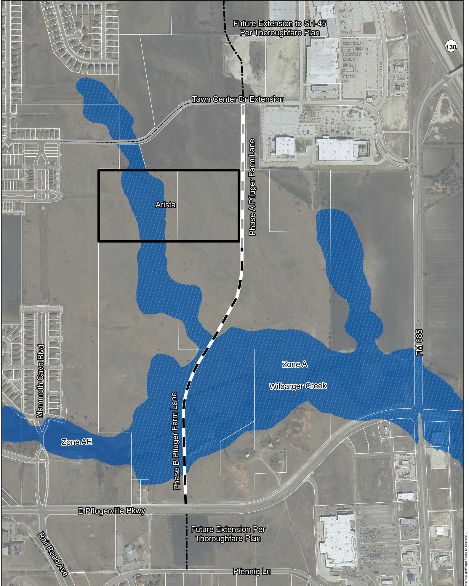
PFLUGER FARM LANE ULTIMATE ROAD ALIGNMENT FROM TOWN CENTER DR TO E. PFLUGERVILLE PKWY
