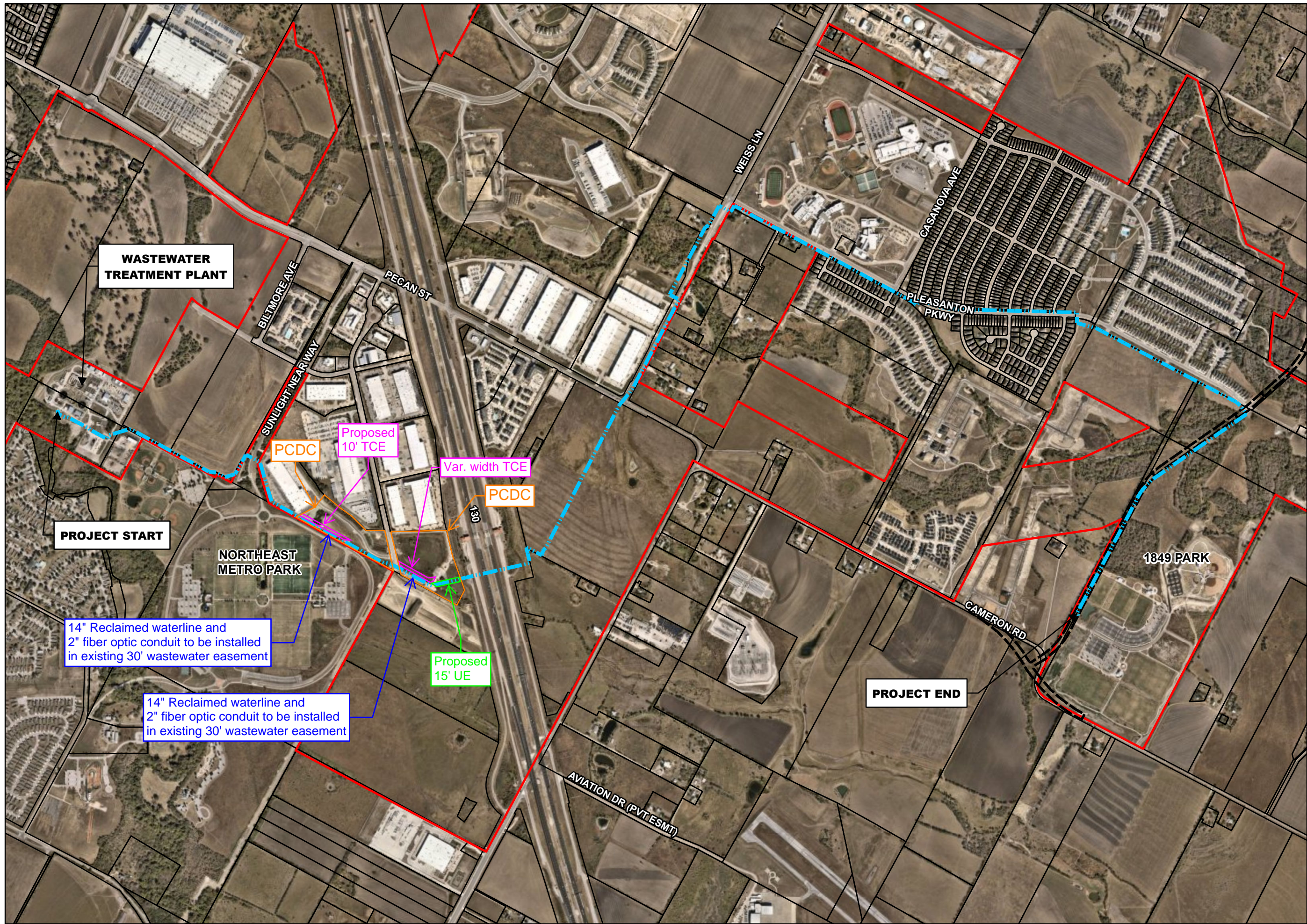
RECLAIMED WATERLINE TO 1849 PARK OVERALL MAP
