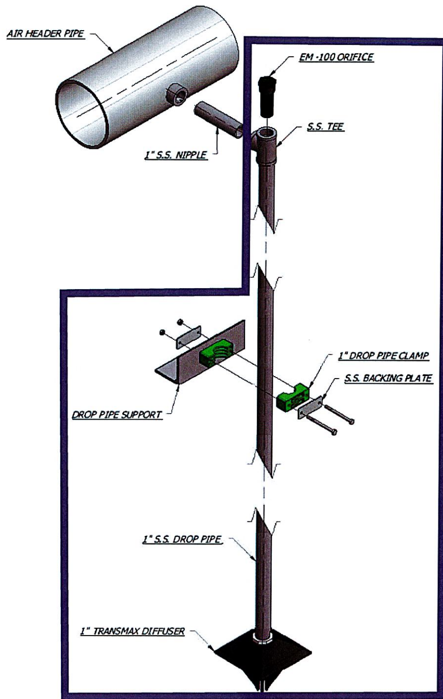
TRANSMAX DIFFUSER ASSEMBLY - TYPICAL
