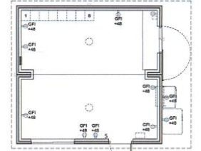
FLOOR PLAN SCALE: NOT TO SCALE
