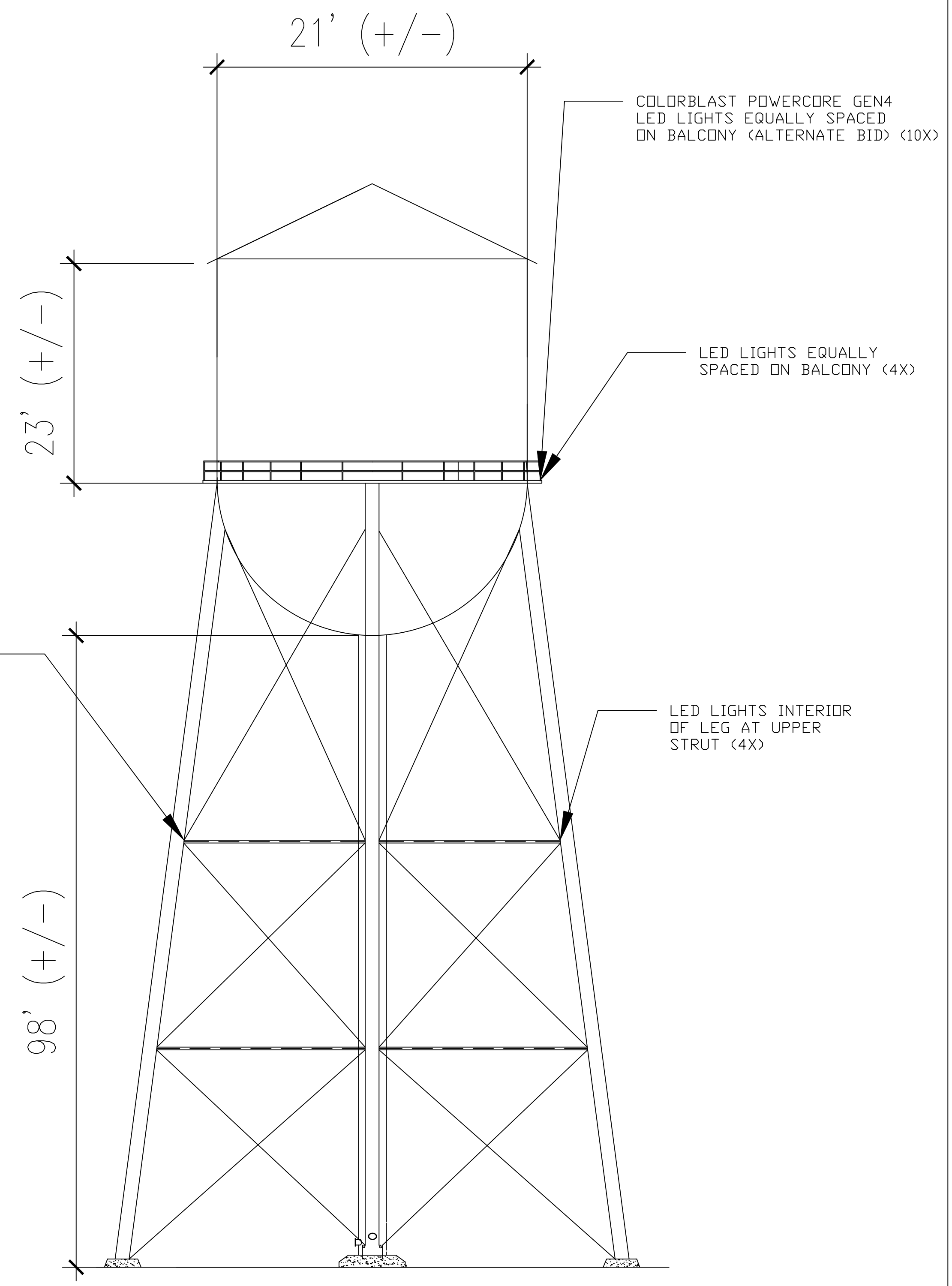
ELEVATION NOT TO SCALE
