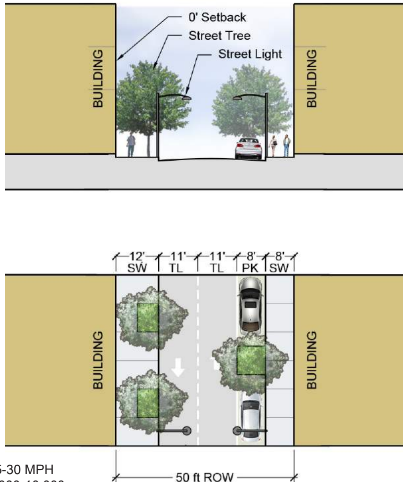
EXHIBIT H4: PUBLIC OR PRIVATE STREET SECTION - 50' ROW (A STREET OR B STREET)
